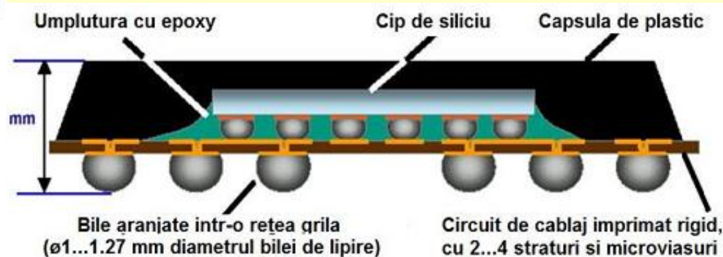
Flip cip BGA
